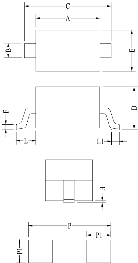
Land Pattern
